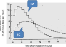
Abbildung 1: Absorptionsrate Insulin, Voag A Variation in absorption of NPH insulin due to intramuscular injection
